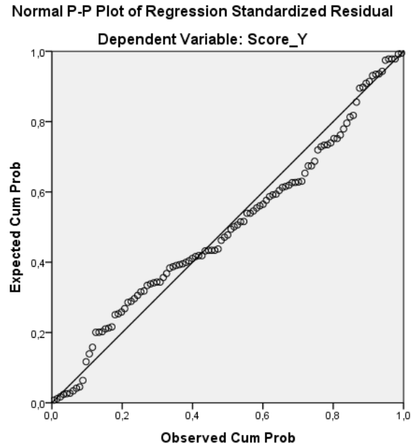
Gambar 4.2 P-P plot Normalitas
